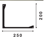
L2 ARSTYL® 200 x 250 x 2000mm
