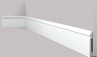
FL2 WALLSTYL® 120 x 15 x 2000 mm
